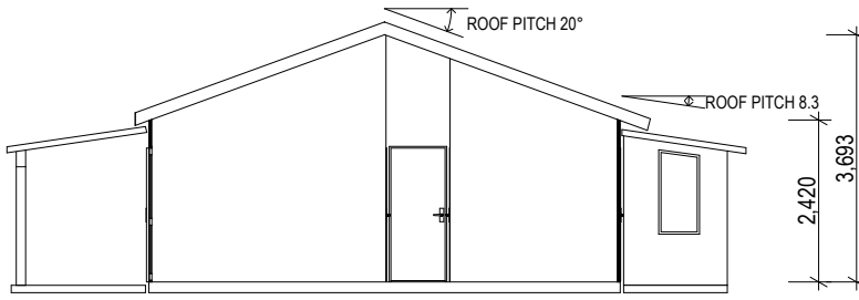
CROSS SECTION
