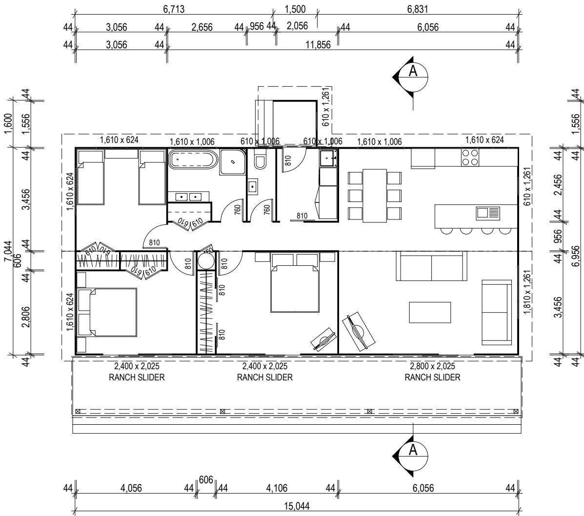
FLOOR PLAN
