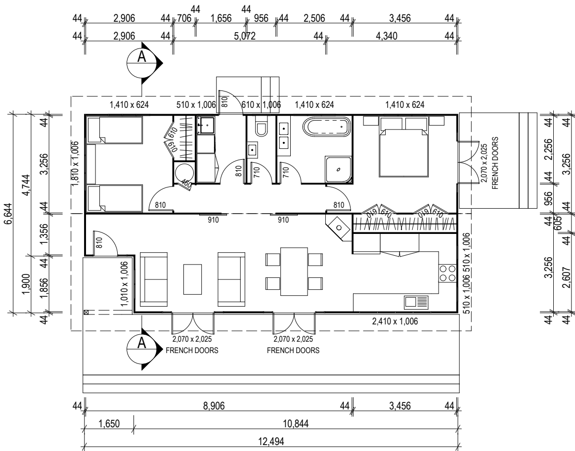
FLOOR PLAN
