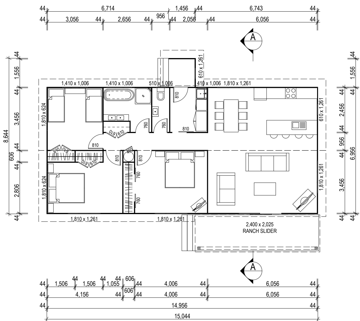
FLOOR PLAN
