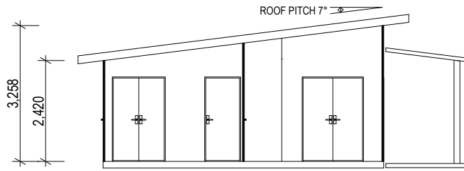
CROSS SECTION
