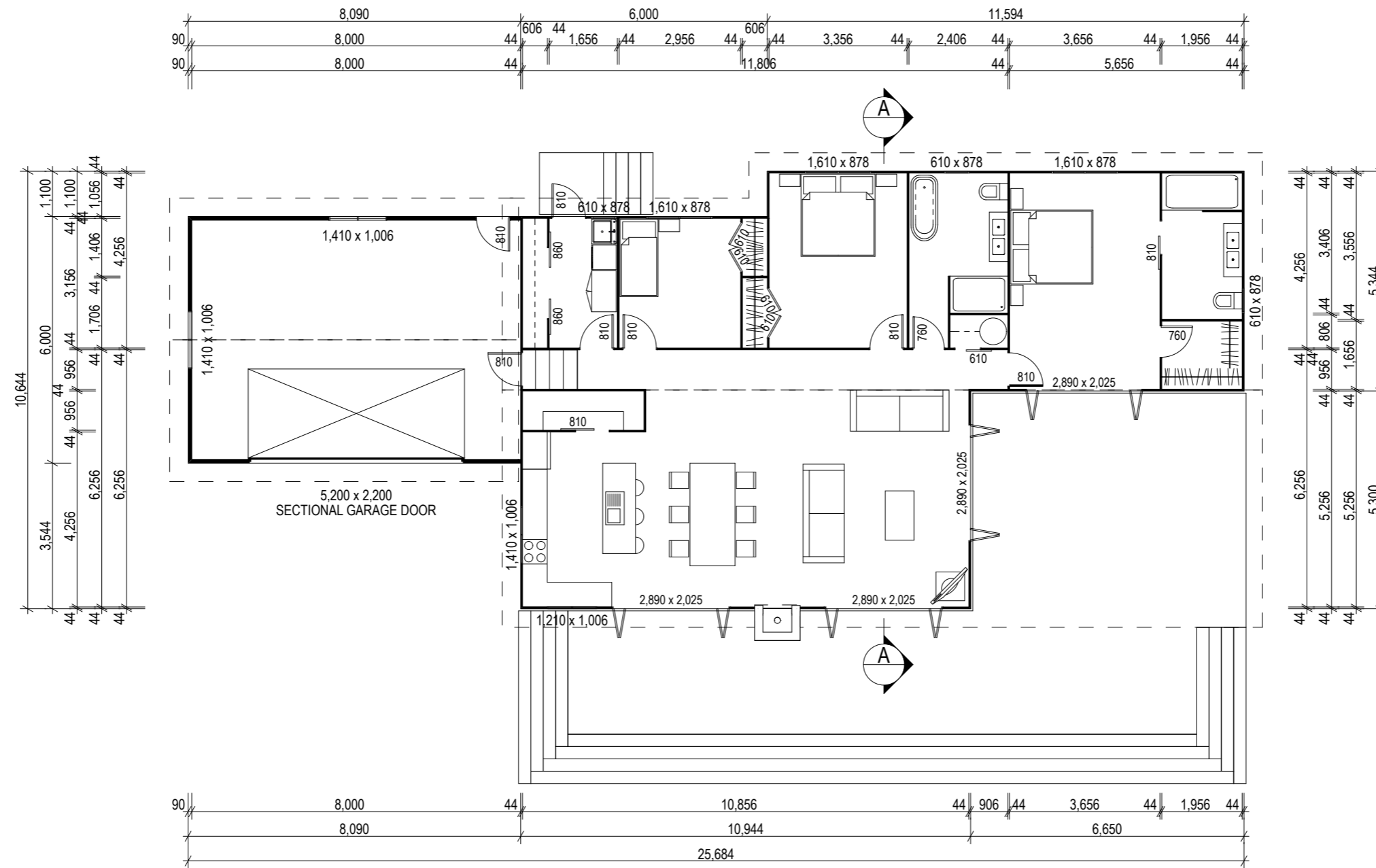
FLOOR PLAN
